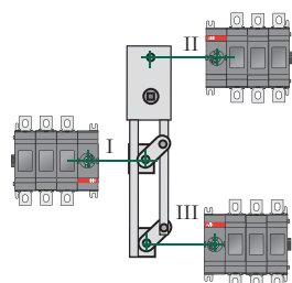
Bypass switches
