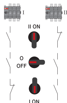
Change-over switches
