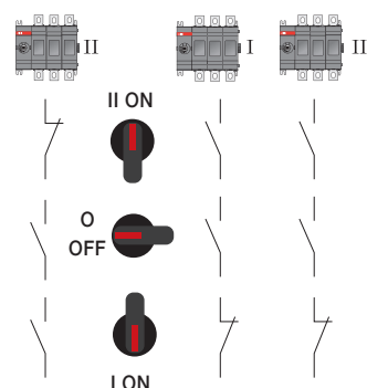
Bypass switches
