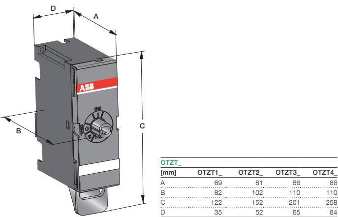
Electrical and mechanical interlock OTZT_
